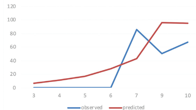
Figure 2. Comparison observed and predicted POI in the validation cohort.
